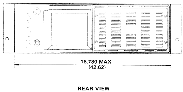
Fig. 6-6. Dimensional drawing.
