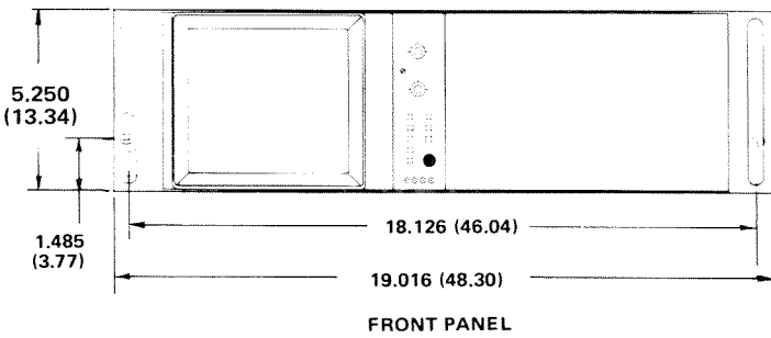
Fig. 6-6. Dimensional drawing.
