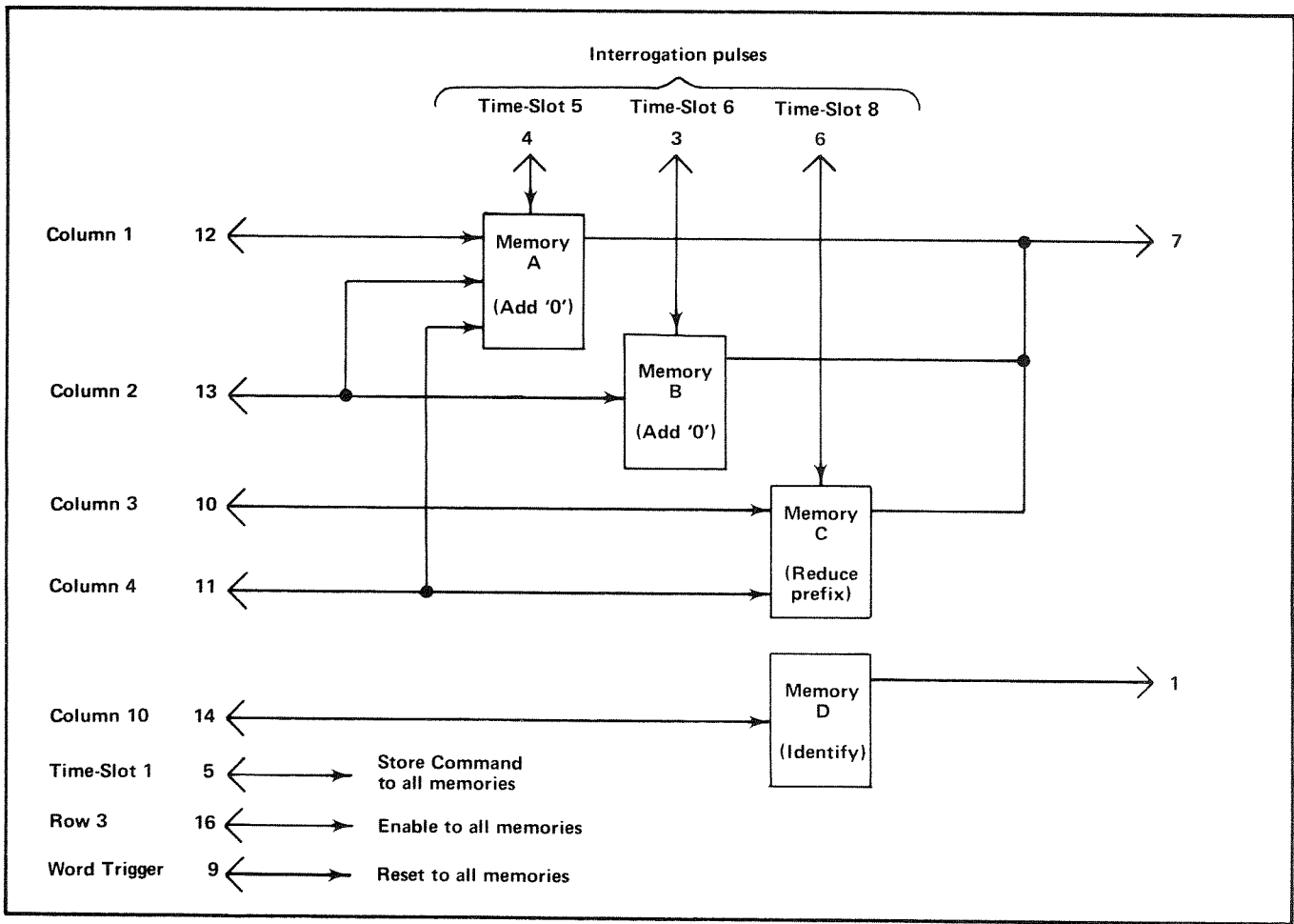
Fig. 4-34. Block representation of memory sequence in U2232.
