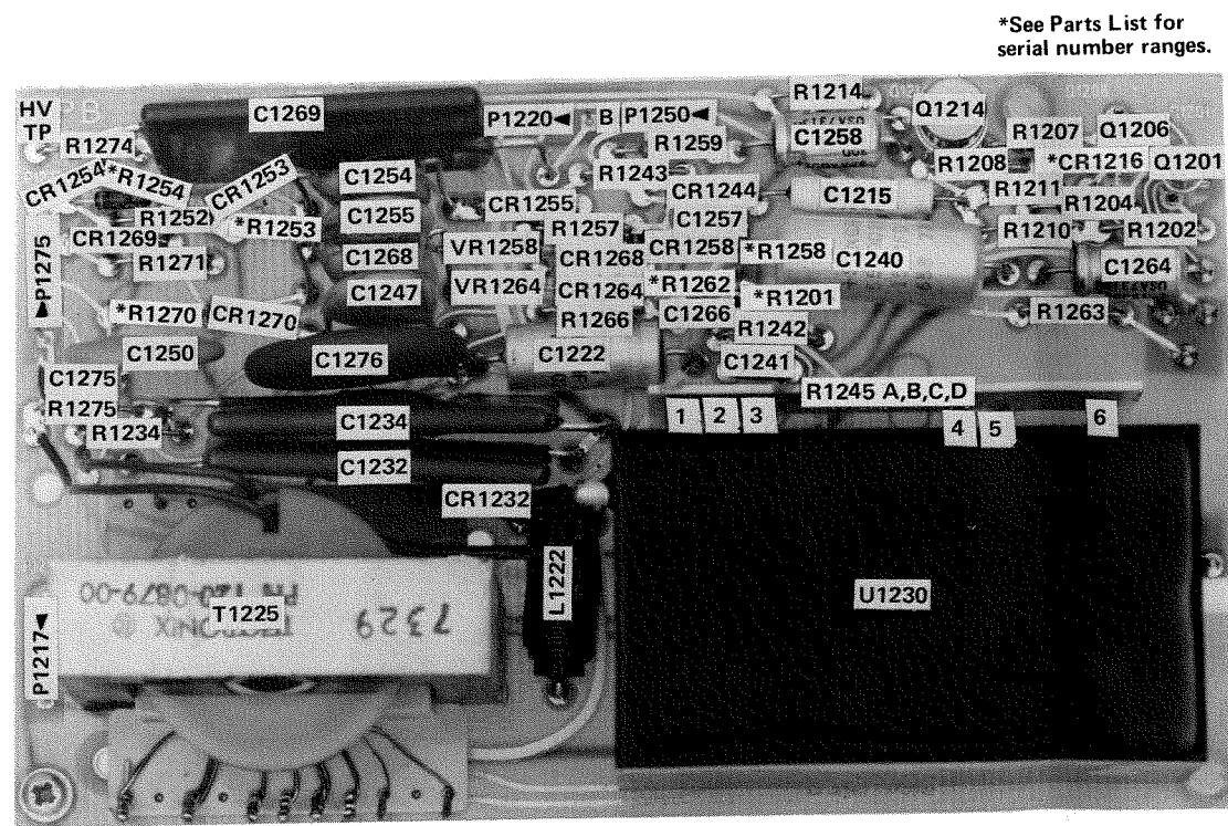
Fig. 8-11A. A9. High Voltage circuit board SN B100000-up.
