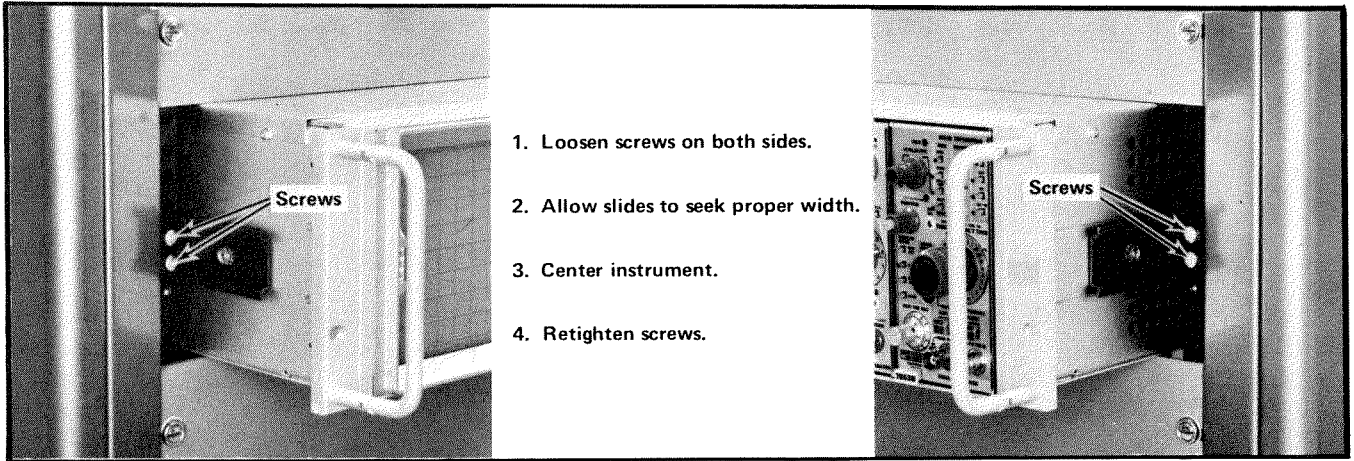
Fig. 6-5. Adjusting the slide-out tracks for smooth sliding action.
