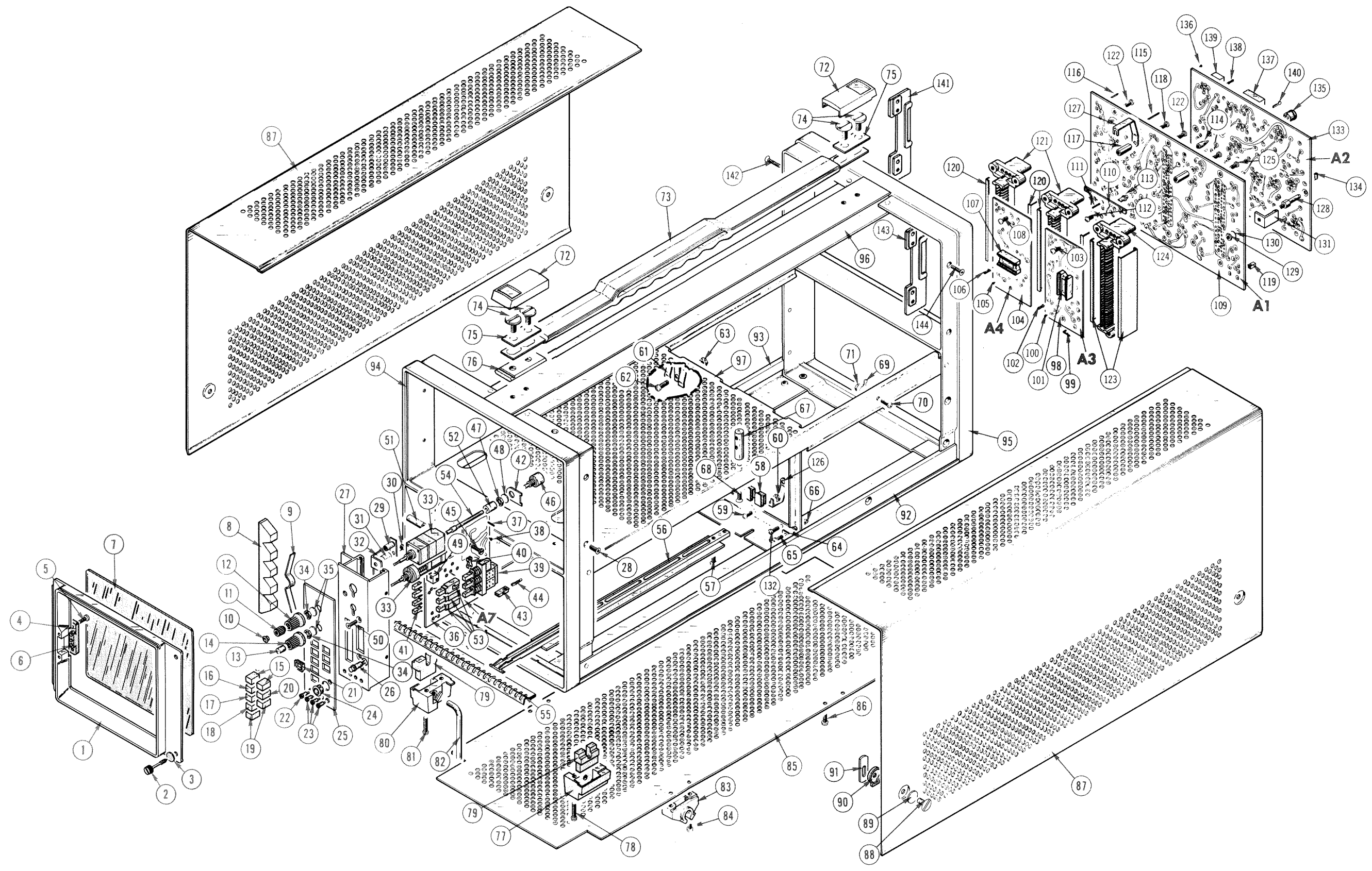
7603/R7603 OSCILLOSCOPE
